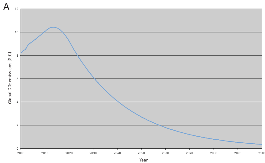
Figure 2.4 CO 2 emissions in reference case: emissions rise at 1.75 per cent annually until 2010, then make a gradual transition to four per cent rate of decline by 2020, continuing through to 2100
