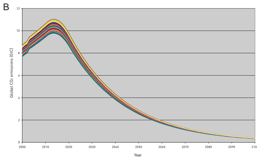
Panel B: Probability envelope generated by 50 model runs with land use emissions defined by a normal distribution with mean 1.5 GtC and standard deviation 0.25 (see Box 2.1).
