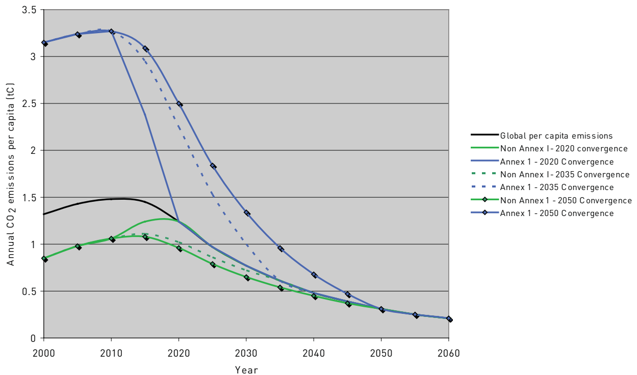
Figure 5.1 Per capita CO 2 emissions globally and for three convergence years (2020, 2035, 2050) for Annex I (developed) and Non-annex I (developing) countries
