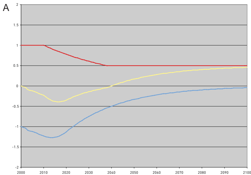
Figure 3.2 Non-CO 2 forcings
