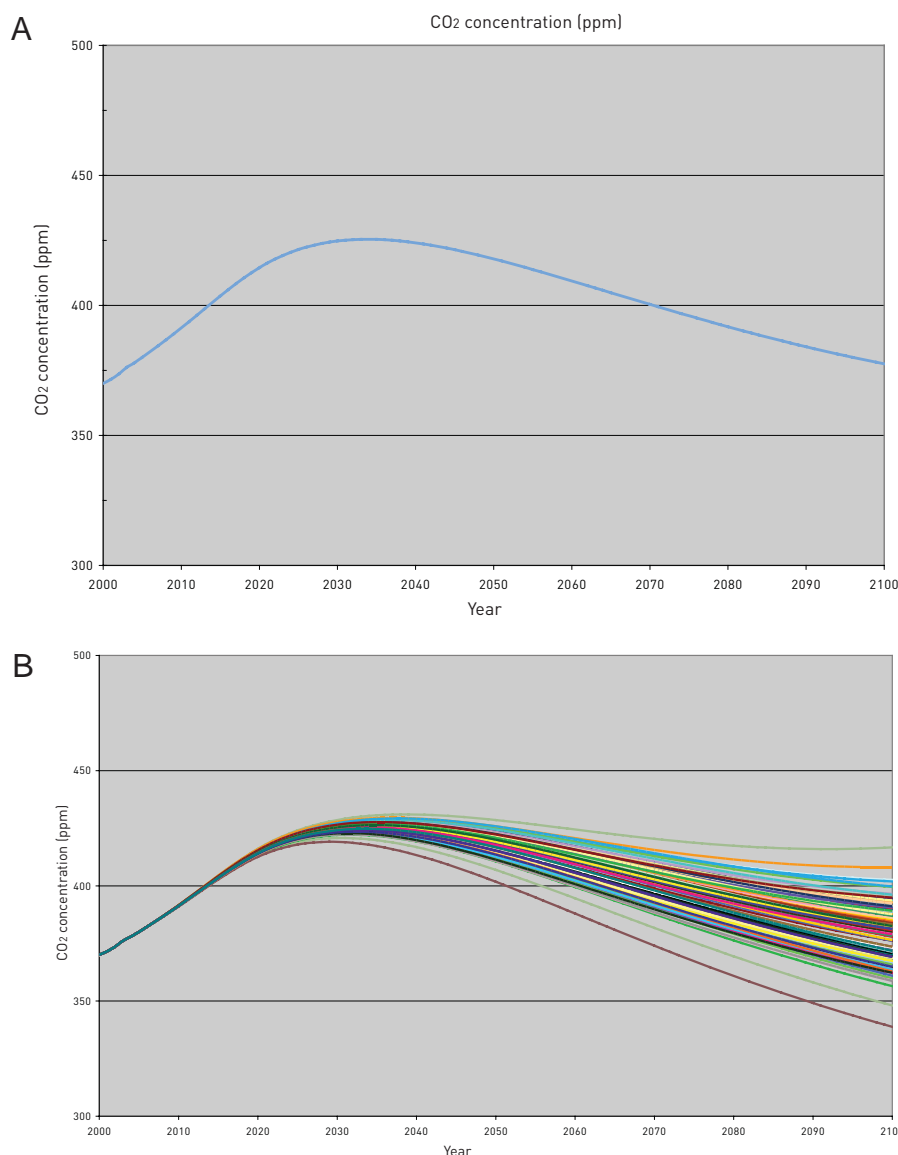
Figure 3.1 Atmospheric CO 2 concentration for emissions reference scenario (see Figure 2.5)
